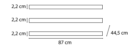
SET 3 PIANETTI ARMADIO SCORREVOLE L. 179 3 WOODEN SHELVES FOR WARDROBE WITH SLIDING DOORS L. 179
