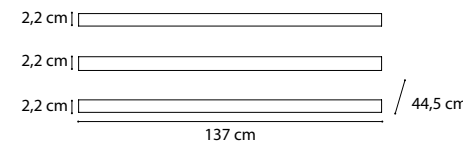
SET 3 PIANETTI ARMADIO SCORREVOLE L. 280 3 WOODEN SHELVES FOR WARDROBE WITH SLIDING DOORS L. 280
