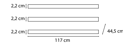
SET 3 PIANETTI ARMADIO SCORREVOLE L. 240 3 WOODEN SHELVES FOR WARDROBE WITH SLIDING DOORS L. 240
